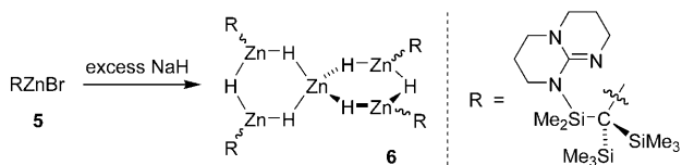
Scheme 1. Synthesis of oligomeric organozinc hydride species 6 from alkylzinc bromide 5 .
